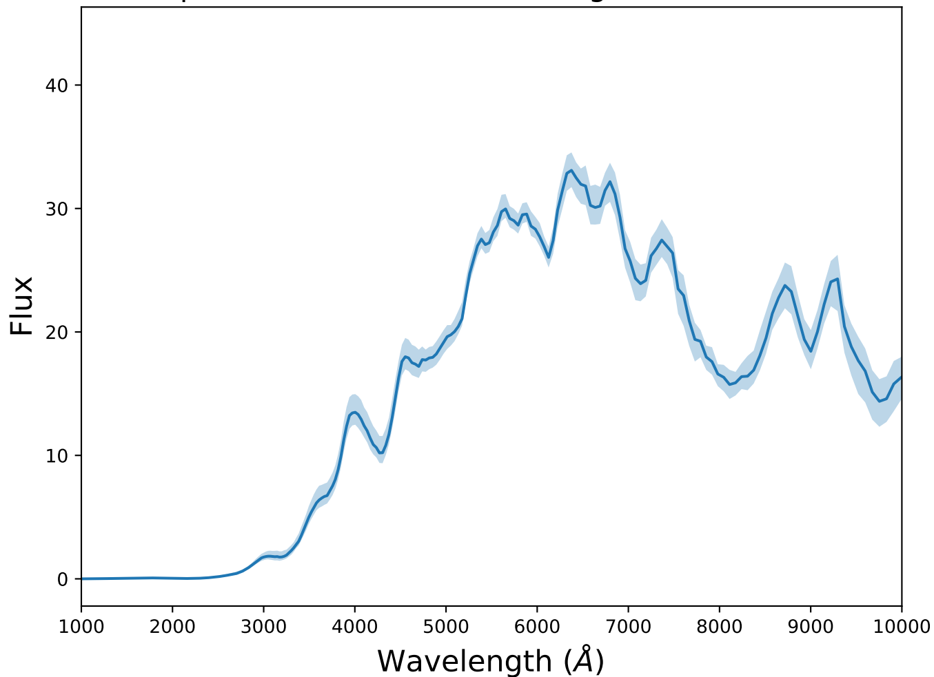
Spectrum 3 for transient 91bg-like at z=0.91
